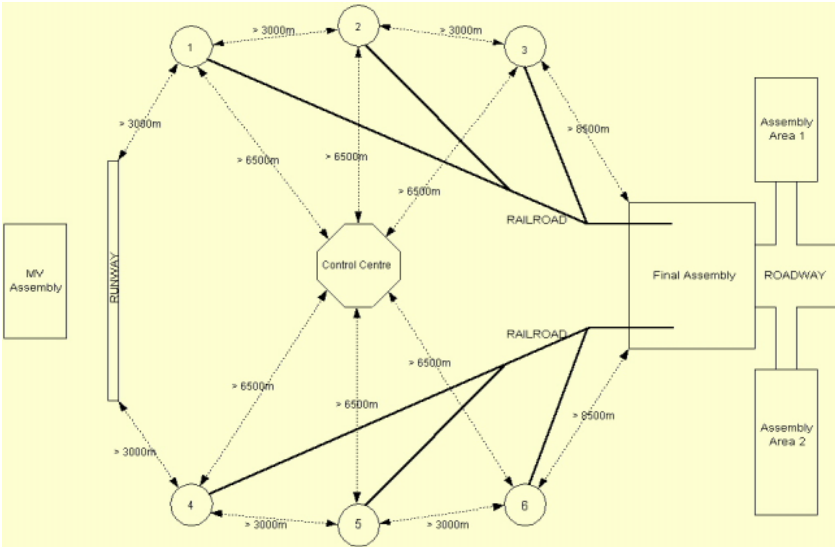
Fig. 1 Proposed Range Head and Launch Pad Layout
