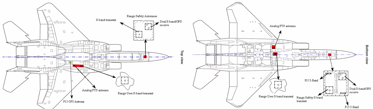
Figure 2. Antenna Locations on the F-15B
