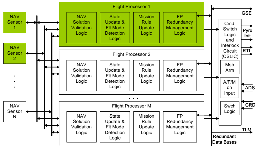
Figure 8. Phase III AFSS Hardware Configuration
