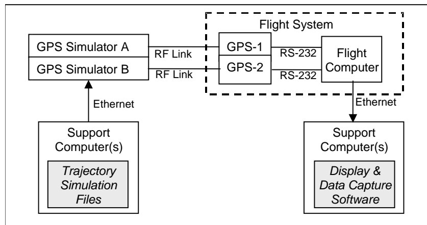
Figure 6. Phase II WFF Simulation Lab Test Configuration
