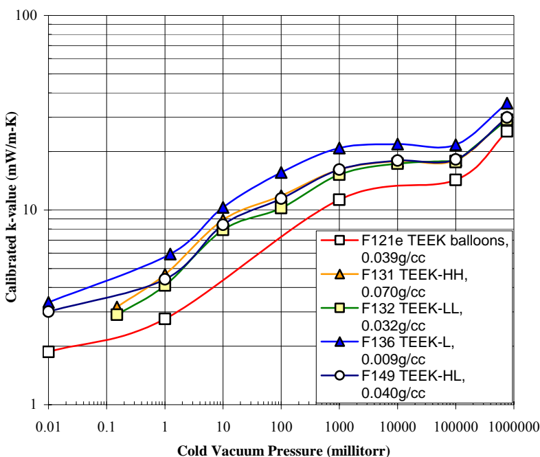
Figure 2. Thermal Conductivity of TEEK-H and TEEK-L series foams under full range of vacuum pressures.
